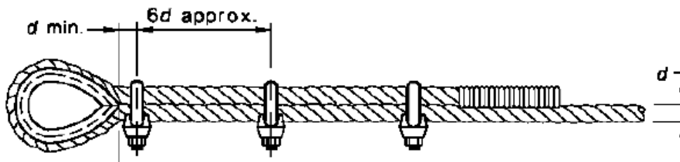
Figure 1: Normal thimble
