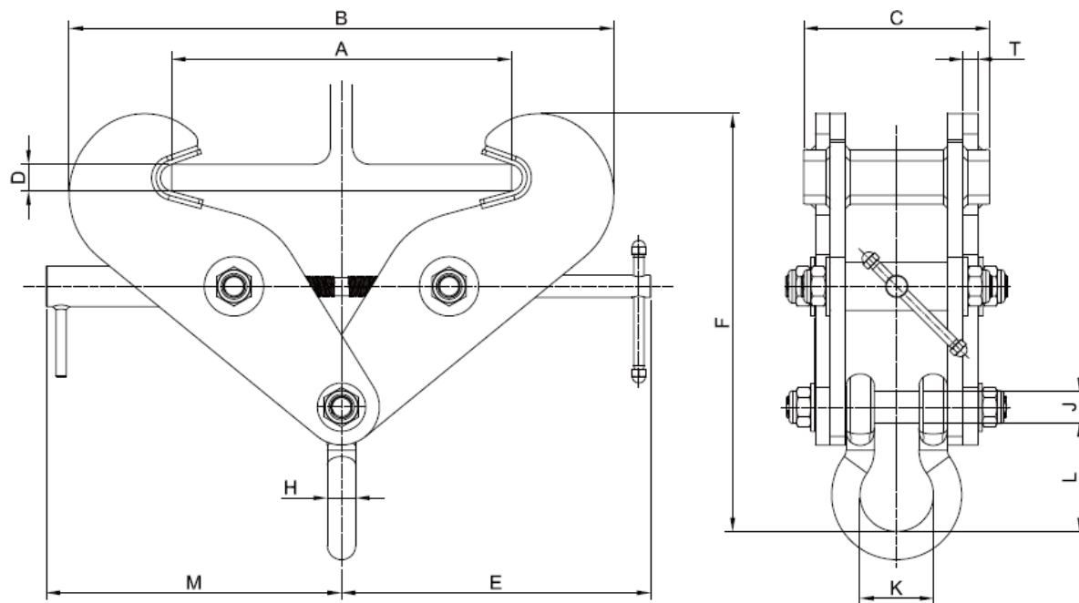
Technical Drawing 15t and 20t
