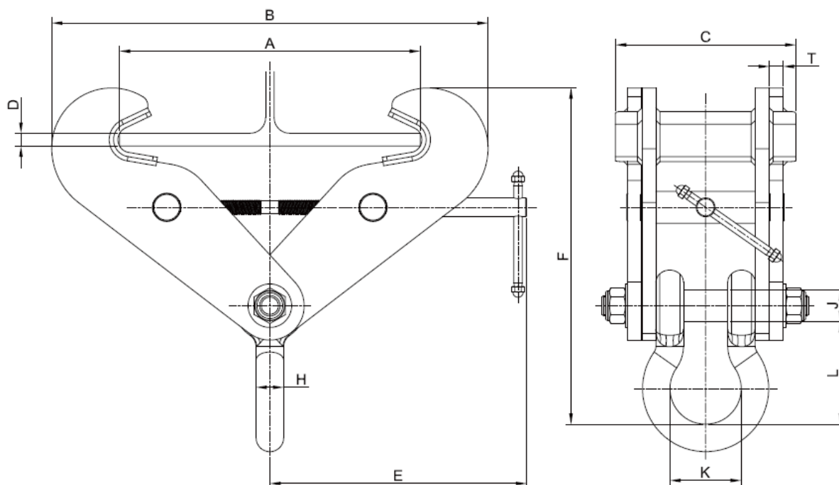
Technical Drawing 10t
