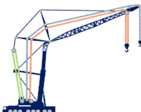
Mobile/Telescopic Crane: Hoist/Auxiliary Hoist Rope
